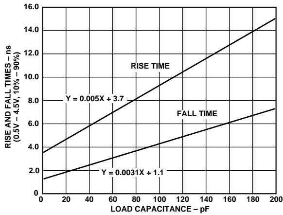
Figure 28. Typical Output Rise Time (10%–90% V_{DD} ) vs. Load Capacitance ( V_{DD} = 5 V )
