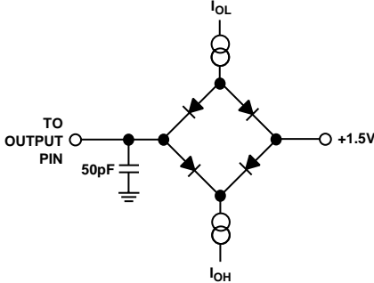
Figure 25. Equivalent Device Loading for AC Measurements (Includes All Fixtures)
