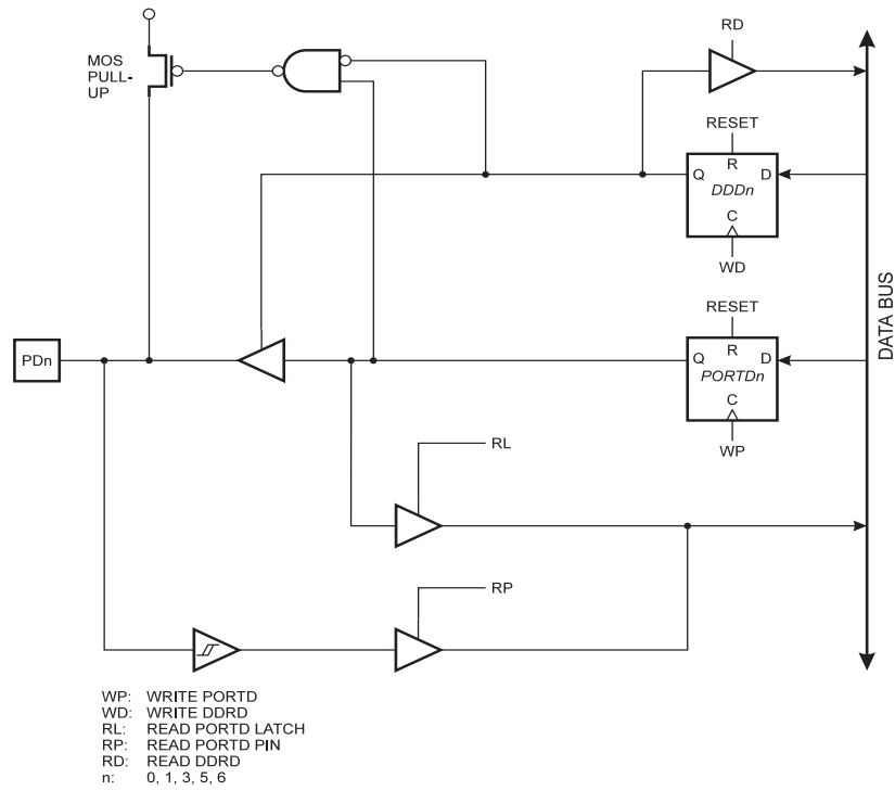
Figure 28. PORTD Schematic Diagram (Pins PD0, PD1, PD3, PD5 and PD6)
