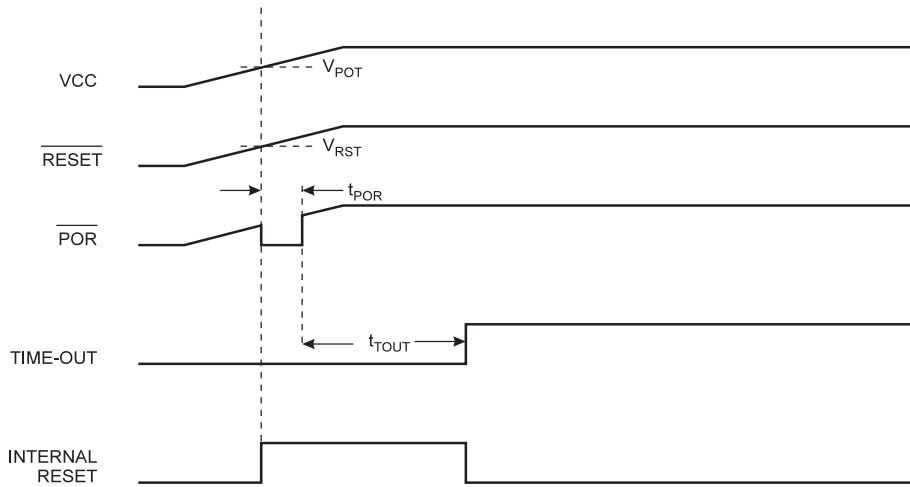
Figure 15. MCU Start-Up, \overline{RESET} Tied to V_{CC} or Unconnected. Slowly Rising V_{CC}
