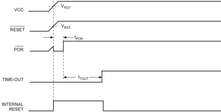
Figure 14. MCU Start-Up, \overline{RESET} Tied to V_{CC} or Unconnected. Rapidly Rising V_{CC} .
