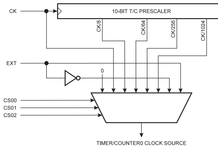
Figure 19. Timer/Counter0 Prescaler
