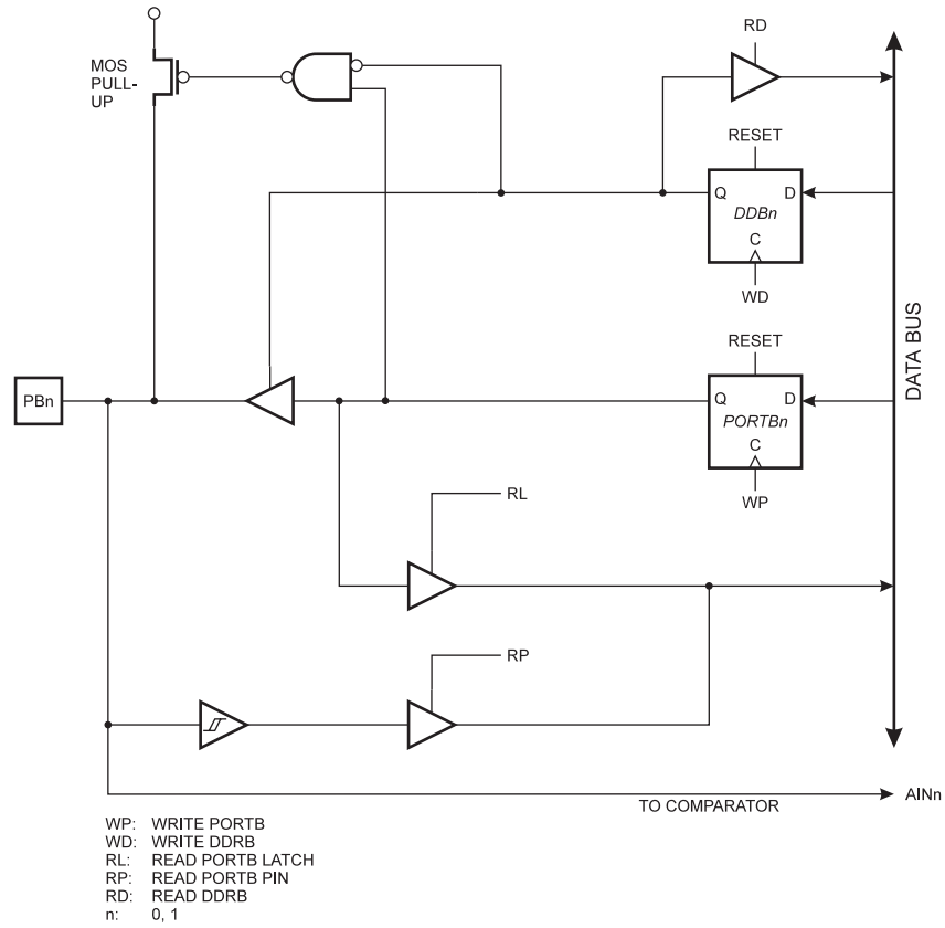
Figure 23. PORTB Schematic Diagram (pins PB0 and PB1)
