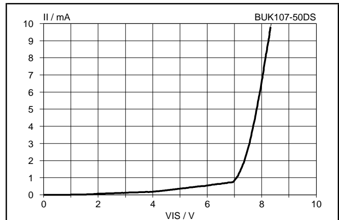
Fig.12. Typical input clamping characteristic. I_i = f(V_{IS}) ; normal operation, T_j = 25 °C.
