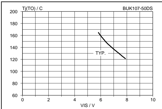
Fig.8. Typical overtemperature protection threshold. T_{j(TO)} = f(V_{IS}) ; condition: V_{DS} = 10 V
