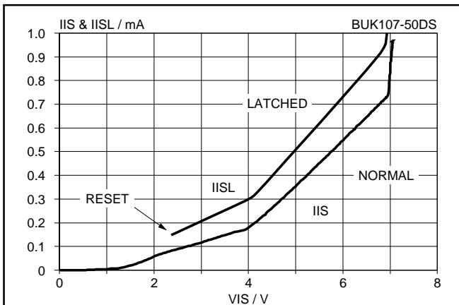
Fig.9. Typical DC input characteristics, T_j = 25 °C. I_{IS} & I_{ISL} = f(V_{IS}) ; normal operation & protection latched
