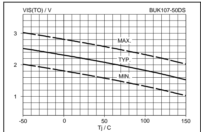
Fig.11. Input threshold voltage. V_{IS(TO)} = f(T_j) ; conditions: I_D = 1 mA; V_{DS} = 5 V
