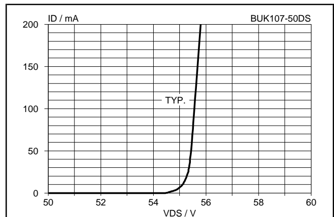
Fig.13. Overvoltage clamping characteristic, 25 °C. I_D = f(V_{DS}) ; conditions: V_{IS} = 0 V; t_p \leq 300 μs
