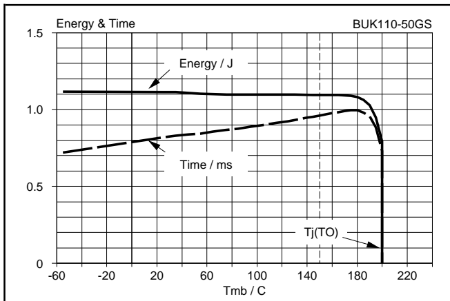
Fig. 14. Typical overload protection characteristics. Conditions: V_{DD} = 13\text{ V} ; V_{IS} = 10\text{ V} ; SC\text{ load} = 30\text{ m}\Omega
