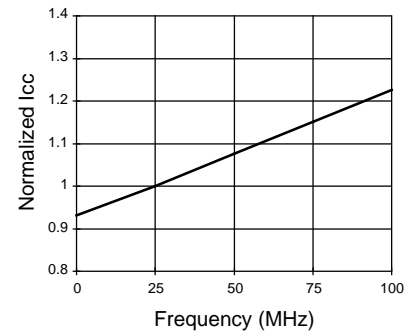
Normalized Icc vs Freq.
