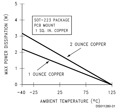
FIGURE 6. Maximum Power Dissipation vs T_{\text{AMB}} for the SOT-223 Package
